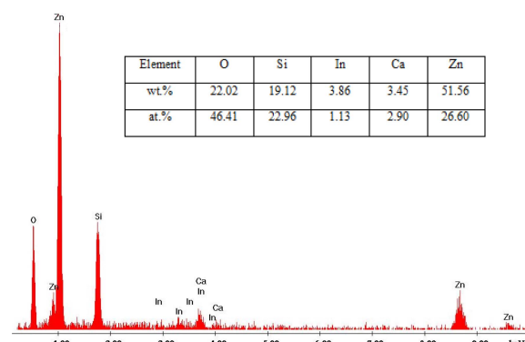
Fig. 4. A typical EDX spectrum of 2.0 at % In doped ZnO thin film.
