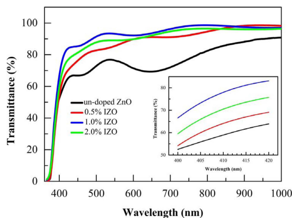
Fig. 3. Optical transmittance spectra of the undoped ZnO and IZO films in the wavelength range of 350-1000 nm.
