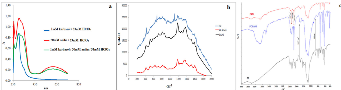
Figure 3. a) UV-vis, b) Raman and c) FT-IR spectrums of PC, PANI and PC -PANI films.
