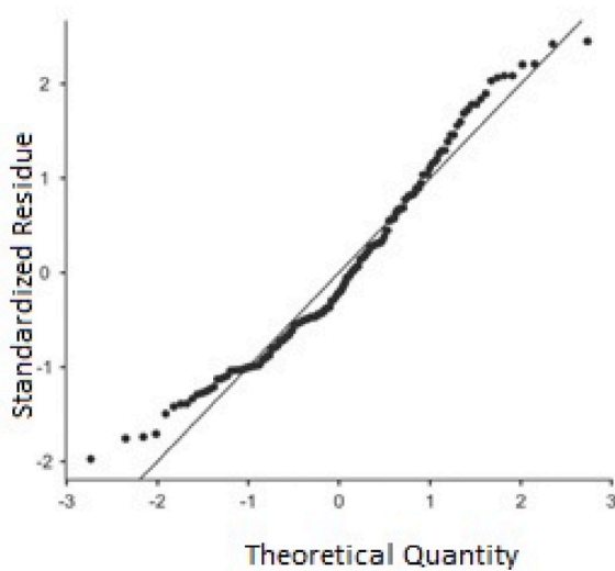
Fig. 7. Q-Q plot showing the distribution of marginal gap values.
