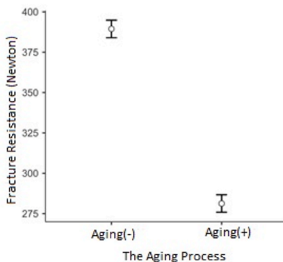
Fig. 17. Graphical representation of the fracture resistance values of aging and non-aging process temporary crowns, regardless of material type (95% confidence interval).
